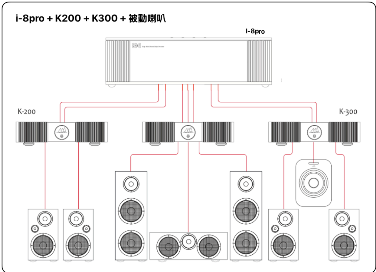
圖五：i-8pro + K-200x1 + K-300x2
